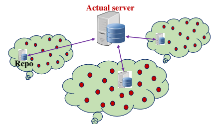
Fig. 3: The proposed CCN architecture.
